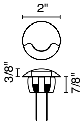
1 x 120° beam
