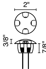
4 x 20° beam
