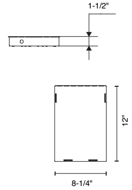
Remote Driver Box (Do not mount on top of BINA body)
