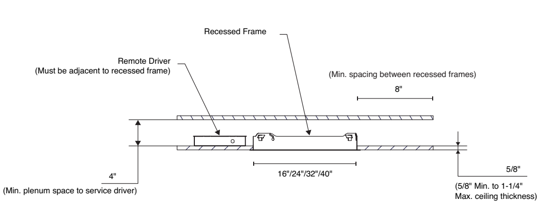
Ceiling to Plenum - Spacing Guide
