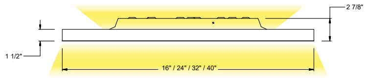
Direct / Indirect - Surface Mount
