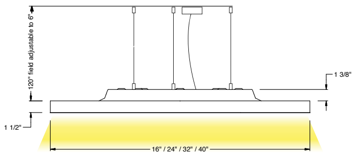
Direct - Ceiling Aircraft Suspension
