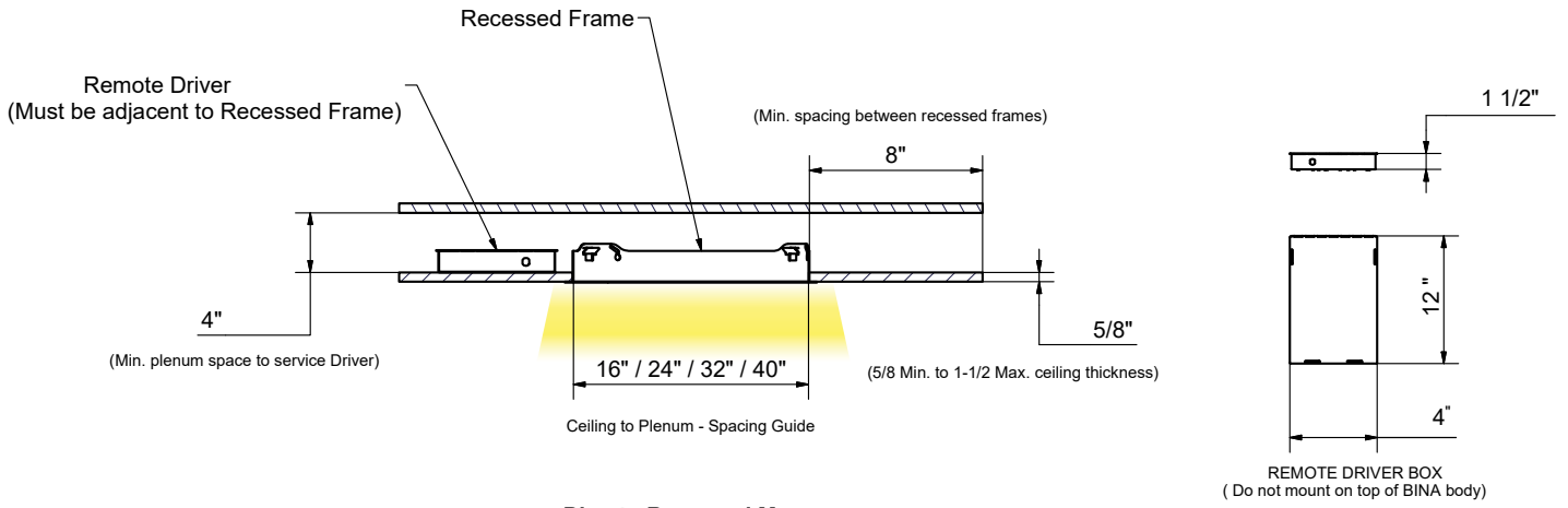
Direct - Recessed Mount
