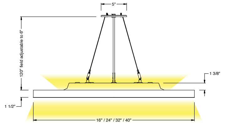
Direct / Indirect - Center Canopy Aircraft Suspension
