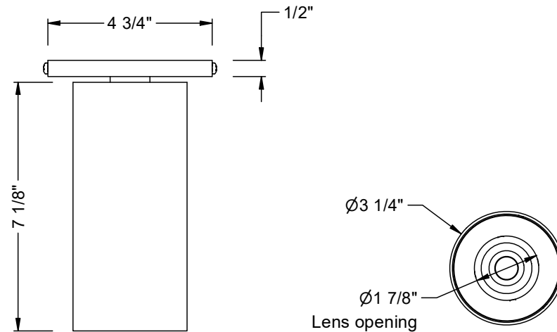
SURFACE MOUNT DIM10 / ELV1 / DMX / CAS (confirm dimming in specsheets)
