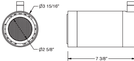
BATWING ASYMMETRIC ELLIPSE 30° X 60°
