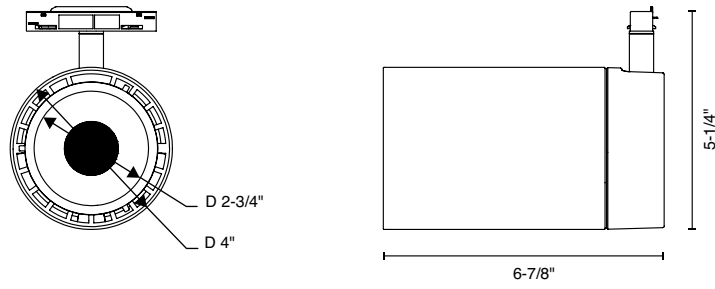
SMT MONOPOINT
