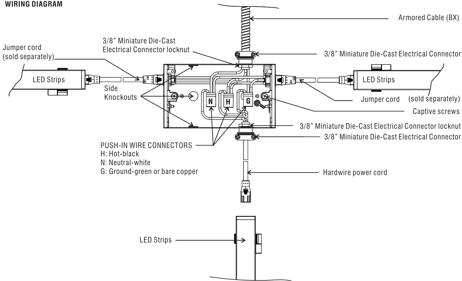
Figure 2: WIRING DIAGRAM
