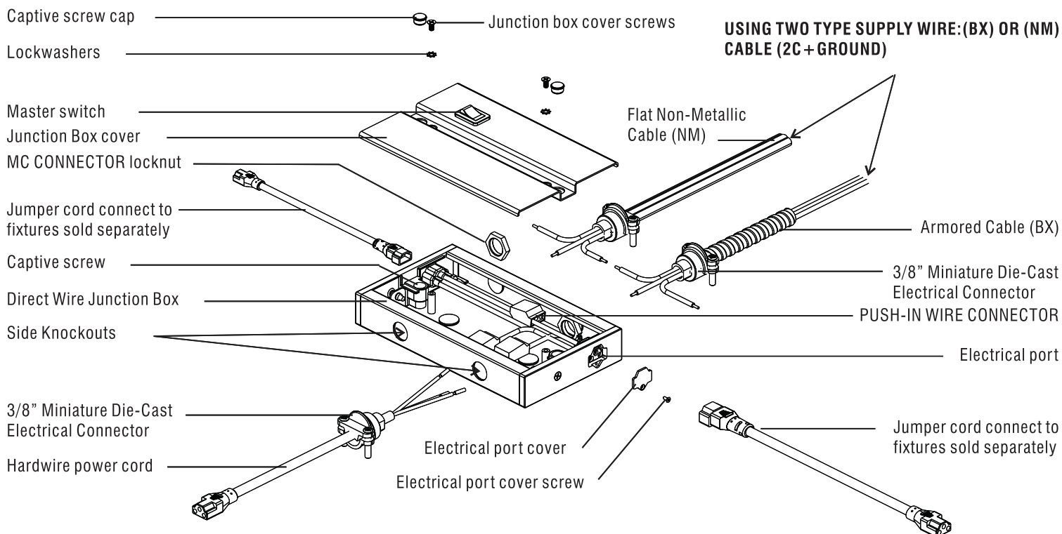
Figure 2: WIRING DIAGRAM
