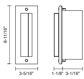
horizontal cover
