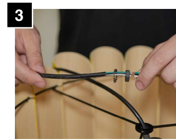
Pass lock washer and nut through cable.
