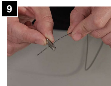
Pass aircraft cable through one hole of strain relief.
