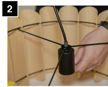
Pull cord until socket bottoms out.
