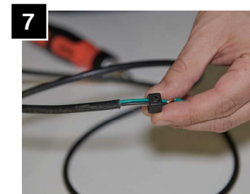
Feed additional strain relief through cord.
