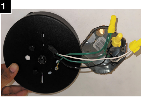
1 Connect Line Voltage and ground wires to building wires. (If necessary, connect Dim wires)
