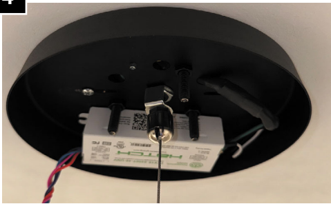
4 Thread aircraft suspension coupler to support fixture's weight.
