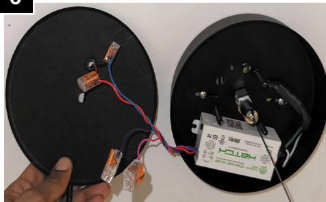
6 While fixture is being supported, connect LED + and LED - wires from fixture to LED + and LED - wires from driver. Note: Wire leads from wep shade may be Black / White. Reference label, DO NOT WIRE TO LINE VOLTAGE.
