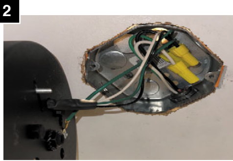
2 Place Line Voltage wires inside junction box.
