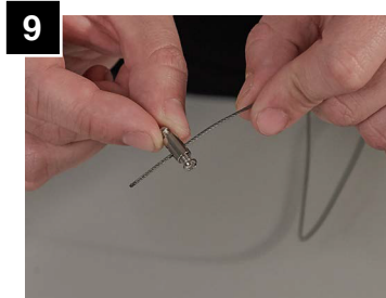
9 Pass aircraft cable through one hole of strain relief.
