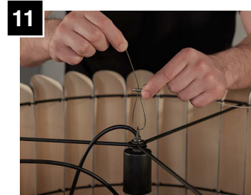
11 Continue to feed aircraft through remaining opening of strain relief.
