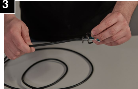
Feed lock washer and nut/balance through cord.
