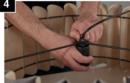
Firmly tighten socket to shade ring.
